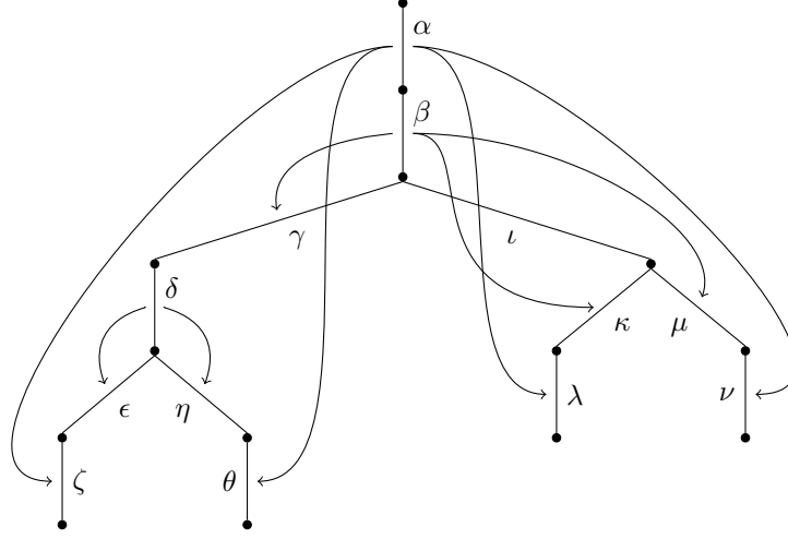
FIGURE 4. Slice tree arising from the derivation tree in Figure 3. Each edge label indicates the slice that induces the edge.
