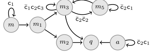
Figure 4. Gadget supporting addition and squaring in S_{\mathbb{N}}
